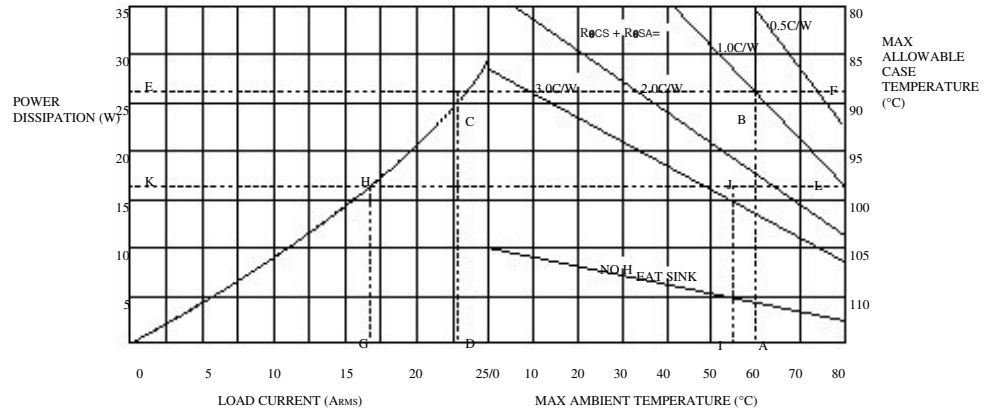
Fig. 2 Thermal operating curves (25 A SSR)
