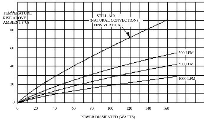
Fig. 6 Typical free-moving air characteristics of a heavy duty heat sink, temperature rise versus power dissipated
