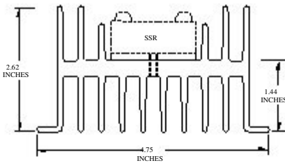
Fig. 5 An end view of a typical heavy duty aluminum heat sink extrusion
