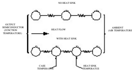
Fig. 1 simplified thermal model. With loads of less than 5 amps, cooling by free flowing air or forced air current around the SSR is usually sufficient. At higher currents it will become necessary to make sure the radiating surface is in good contact with a heat sink. Essentially this involves mounting the base plate of the SSR onto a good heat conductor, usually aluminum. Good thermal transfer between the SSR and the heat sink can be achieved with thermal grease or heat sink compound. Using this technique, the SSR case to heat sink thermal resistance ( R_{\theta CS} ) is reduced to a negligible value of 0.1^{\circ}\text{C/W} (celsius per watt) or less. This is usually presumed and included in the thermal data. The simplified thermal model in Fig. 1 indicates the basic elements to be considered in the thermal design. The values that are determinable by the user are the case to heat sink interface ( R_{\theta CS} ), as previously mentioned, and the heat sink to ambient interface ( R_{\theta SA} ).
