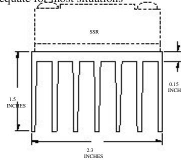
Fig. 3 Typical light duty aluminum heat sink extrusion (end view)
