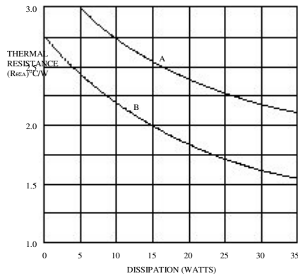
Fig. 4 Typical heat sink characteristics
